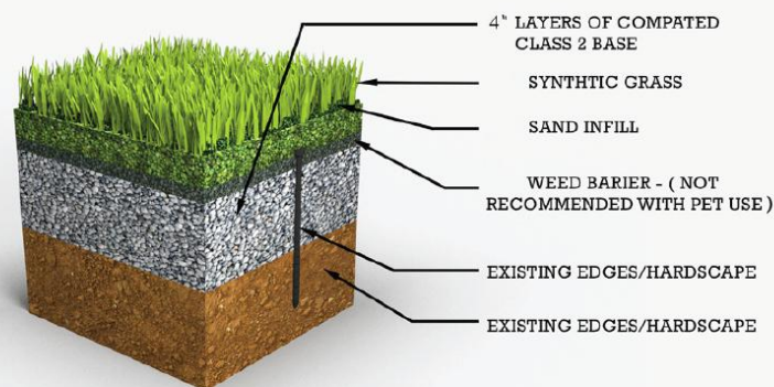
RESIDENTIAL LANDSCAPE ARTIFICIAL GRASS DETAIL
